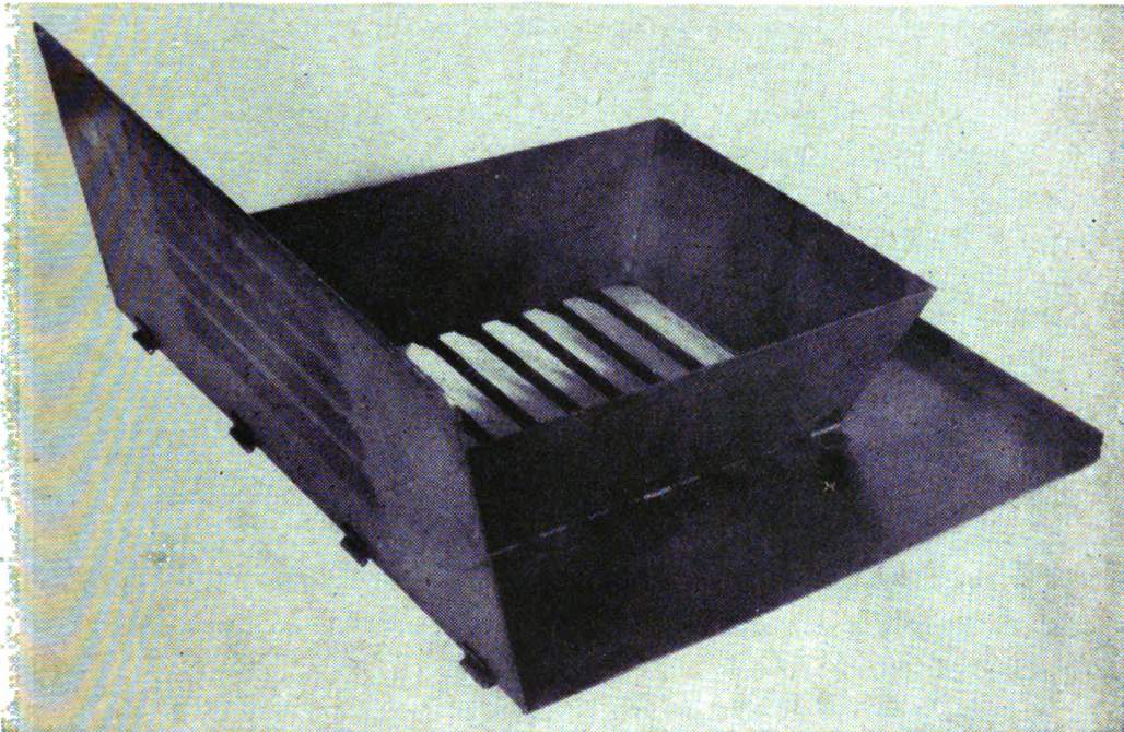
FIGURE 34.—Wood burning grate set up for use.
